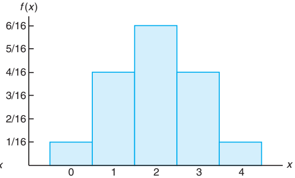
Figure 3.2: Probability histogram.
